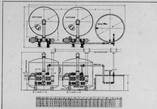
Type C—Double Unit—Sizes 84" to 108"
