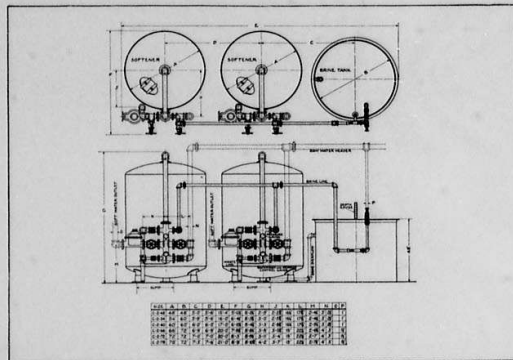
Type C—Double Unit—Sizes 48" to 78"
