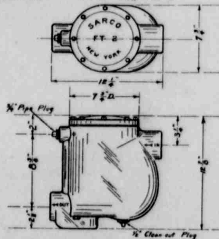
"FT-2" 1 1/2" or 2"
