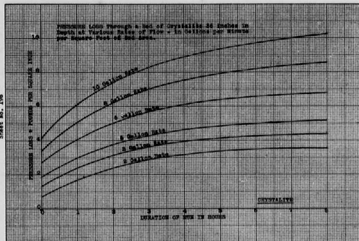
Chart showing Pressure Losses at various rates of flow through Crystallite Zeolite Softeners
