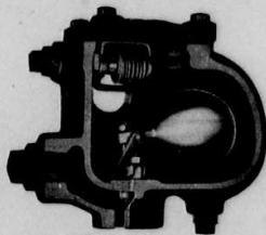
"FT-1" 3/4", 1" or 1 1/4"
