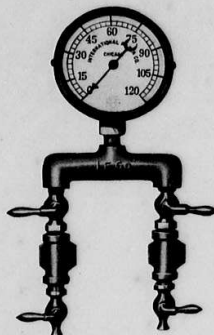
Loss of Head Gauge and Test Cocks
