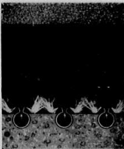
Distribution of wash water by International Umbrella Nozzles. No upward jet action. Full degree distribution in water leaves umbrella cap and is deflected downward to concrete floor.
