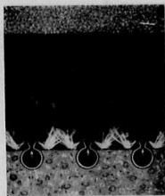
Distribution of wash water by International Umbrella Nozzles. No upward jet action. 140 degree distribution as water leaves umbrella cap and is deflected downward to concrete floor.
