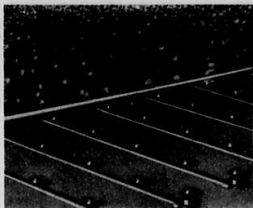
Underdrain system with International Umbrella Distributing Nozzles. The concrete subill blocks the lateral system to provide a smooth floor.
