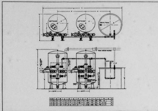
Type C—Double Unit—Sizes 30" to 42"
