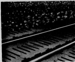
Underdrain system of the International "Wagner Bottom" type. Slotted concrete blocks fit closely in between the distributing laterals.
