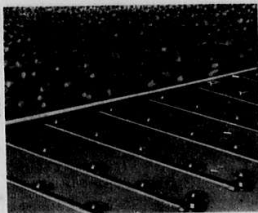
Underdrain system with International Umbrella Distributing Nozzles. The concrete subfill inhibits the lateral system to provide a smooth floor.
