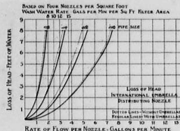
With the International Umbrella Distributing Nozzle there is LESS loss of head or frictional resistance to the passage of wash water with the cone-umbrella cap in place than with cap removed. Perfect distribution with minimum loss of head.
