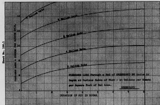
Chart showing Pressure Losses at various rates of flow through Greensand Zeolite Softeners
