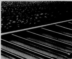
Underdrain system with the lateral pipes perforated on the underside. The concrete subill stops an inch or so beneath the laterals.
