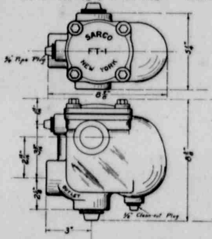
"FT-1" for 3/4", 1" or 1 1/4" DIMENSIONS
