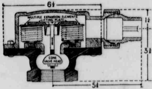
Section of 1 1/4" and 1 1/2" No. 9-3
